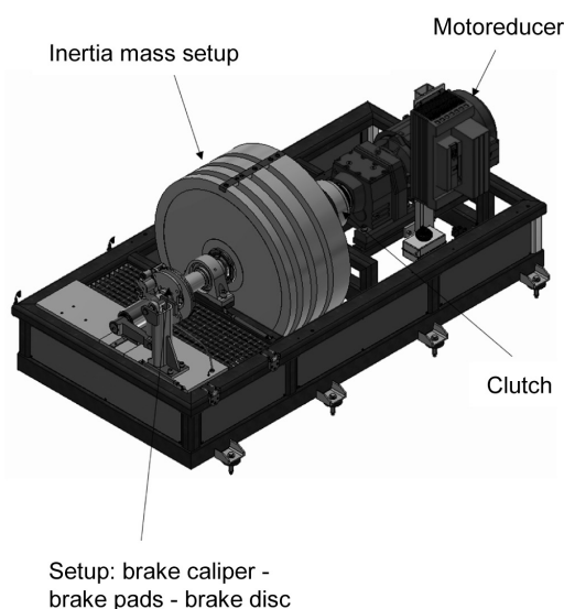
Fig. 3. Dynamic system of the T-33 dynamometer
